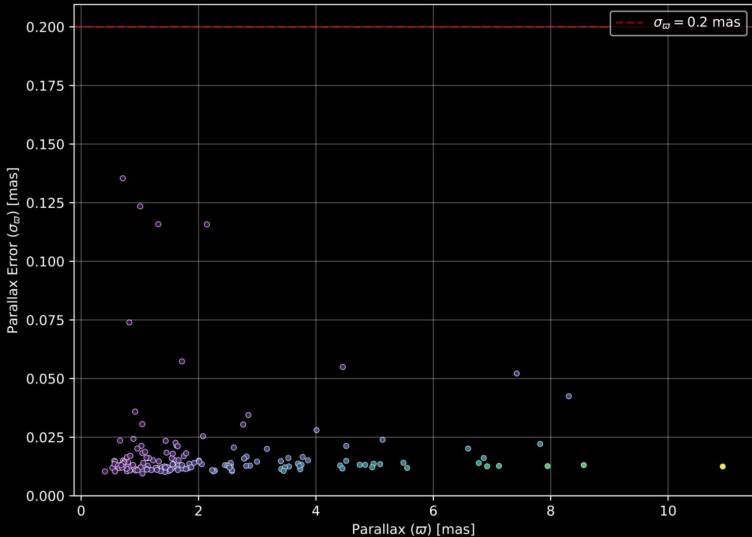
GALAH DR4 Field: [3702] Parallax Quality (n= 161)
