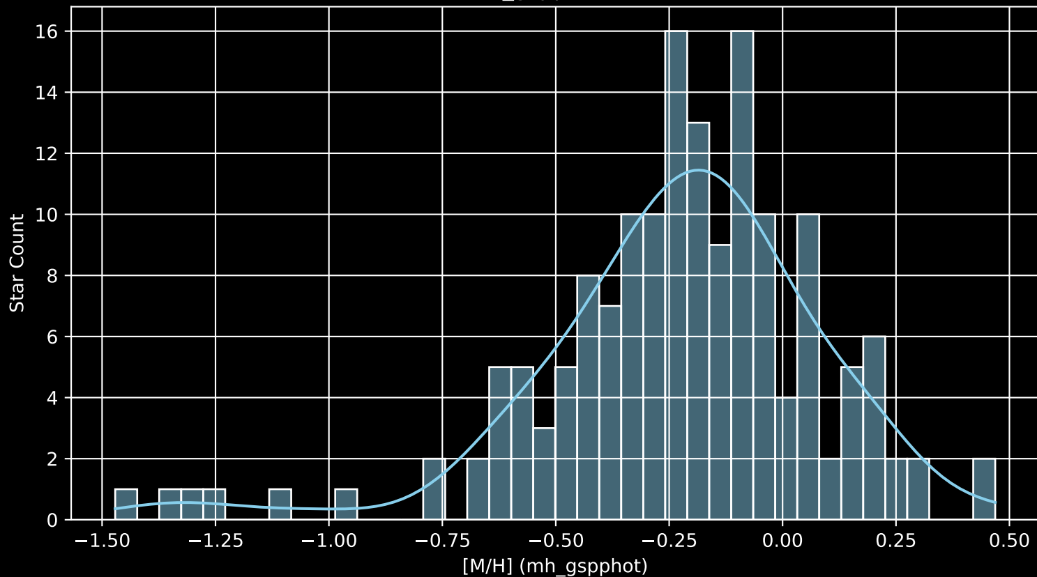
GALAH DR4 Field: [3702] [M/H] (mh_gspphot) (n= 160)
