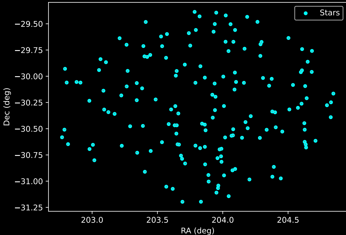
GALAH DR4 Field: [3702] Proper Motion Vectors for Gaia Star Field (n= 161)
