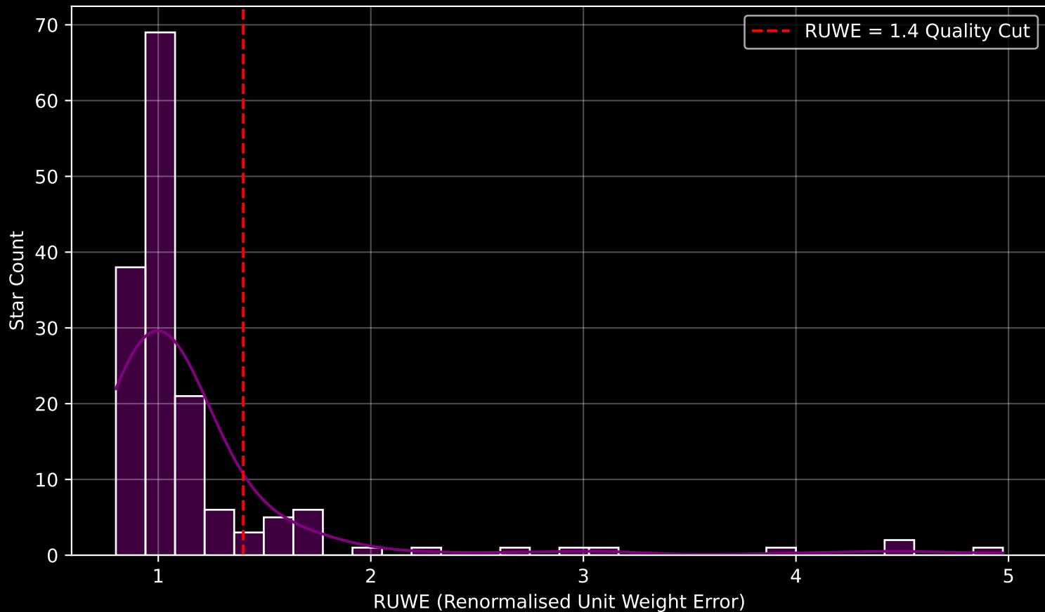
GALAH DR4 Field [3702] RUWE Distribution (n= 157)
