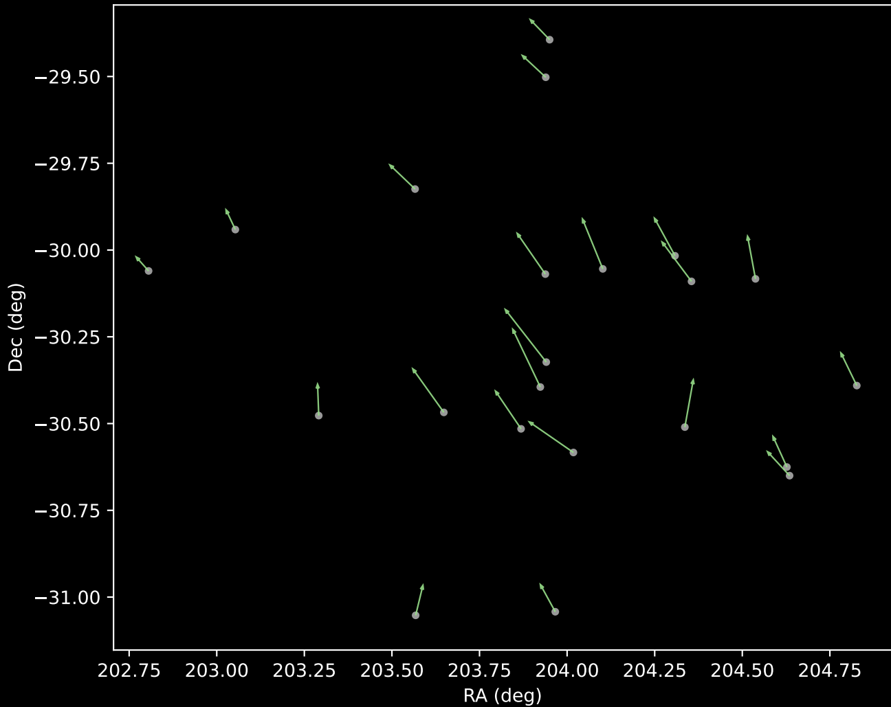
GALAH DR4 Cluster 5 Proper Motion Vectors (n=22)
