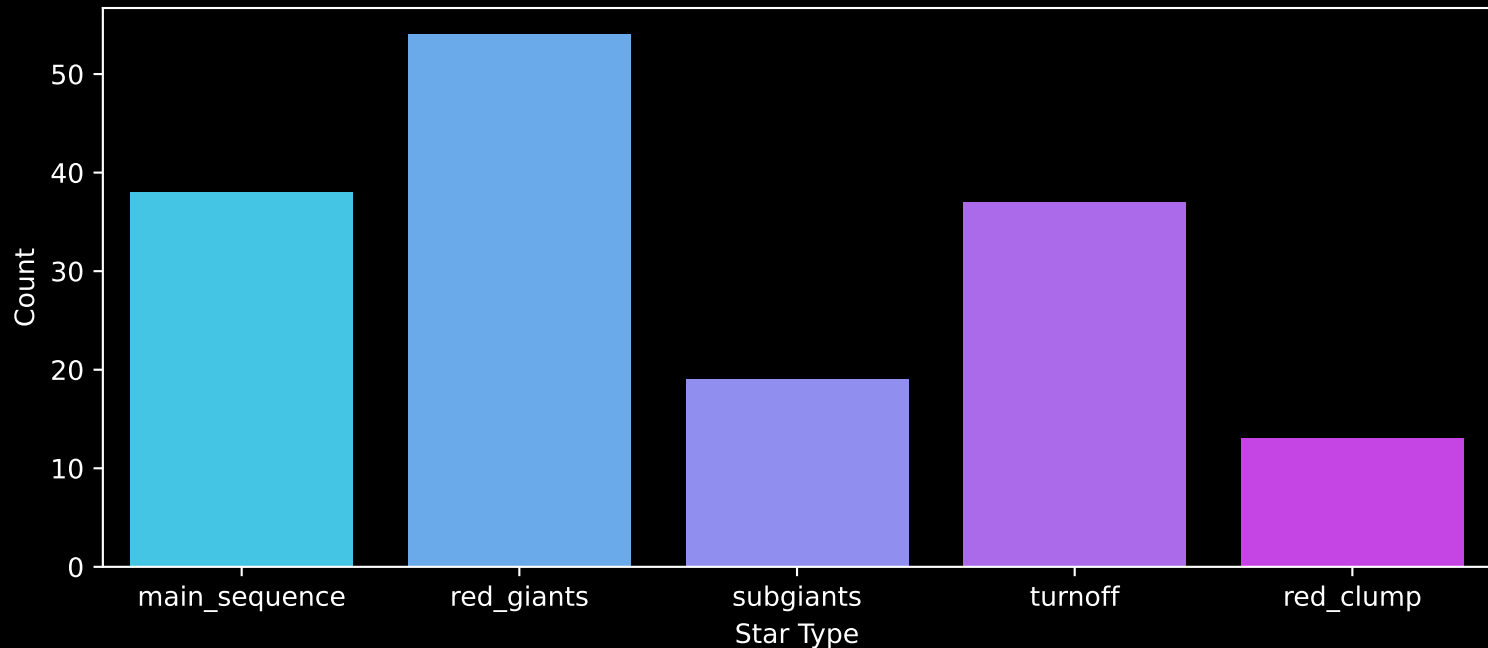
GALAH DR4 Field: [3702] Count plot of Star Type
