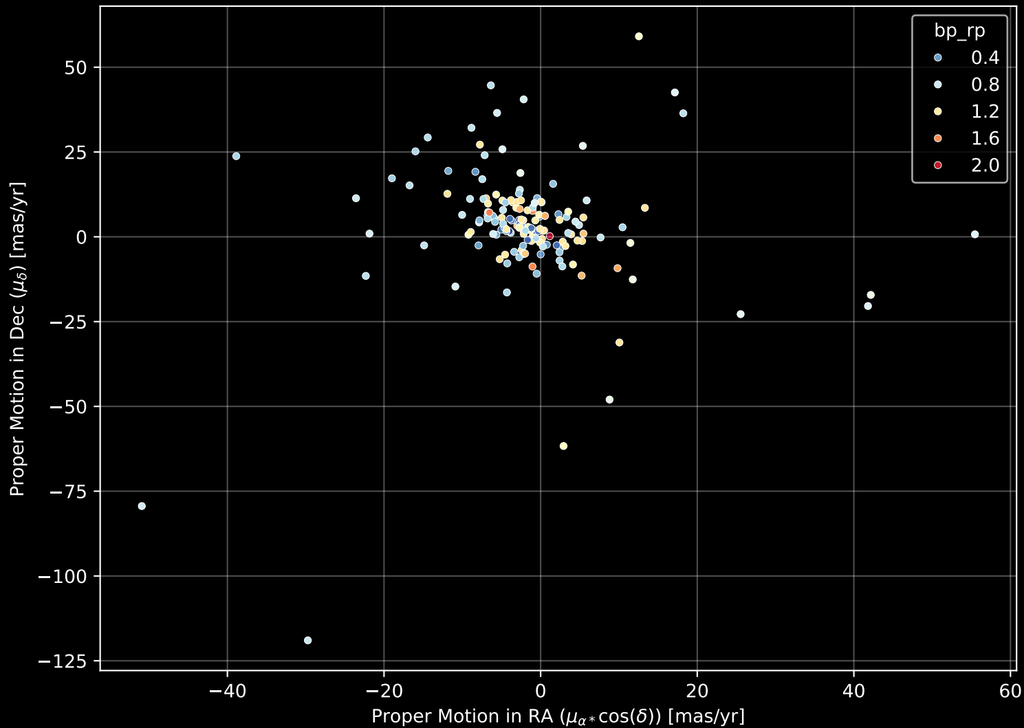
GALAH DR4 Field: [3702] Proper Motion Diagram (n= 161)
